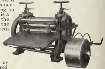
American Bench Roughing Machine with 15-inch rollers
