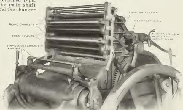
Laureate Models J and T Detailed view from the front and right-hand side. This shows the carriage when provided with the two riding changers, and also the latch for causing all the form rollers to pass, during the up-movement, free of the form. The inking apparatus is the same in both models.
