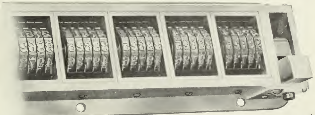
This illustration shows a section of a frame containing ten 5-wheel machines, which was designed to work on a 14x20 inch Gordon Press, and shows model 57 figures, with Spanish spelling above each figure.
