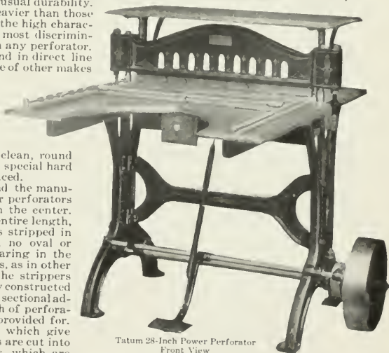
Tatum 28-Inch Power Perforator Front View
