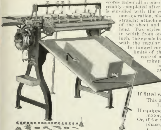
National Rotary Perforator
