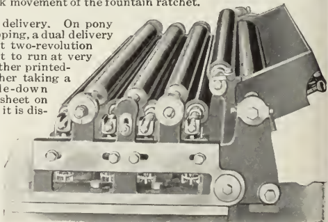
The Premier Fountain is arranged to swing at any angle by loosening one bolt and tightening it again and the fountain is placed above the plate
