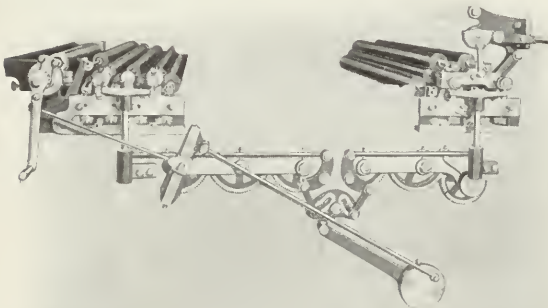
The Unequaled Distribution; note the independent vibratory mechanism
