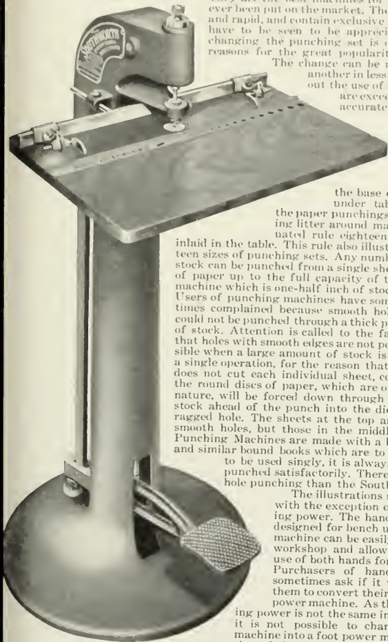
Southworth Punching Machine Foot Power
