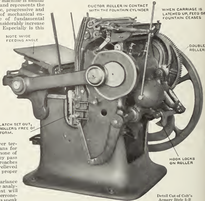
Detail Cut of Colt's Armory Style B
