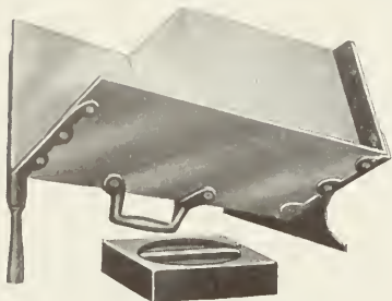
Superior Steel Tableting Press
