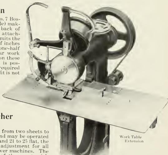
No. 7 Boston Wire Stitcher, showing door open. All working parts and wire always visible
