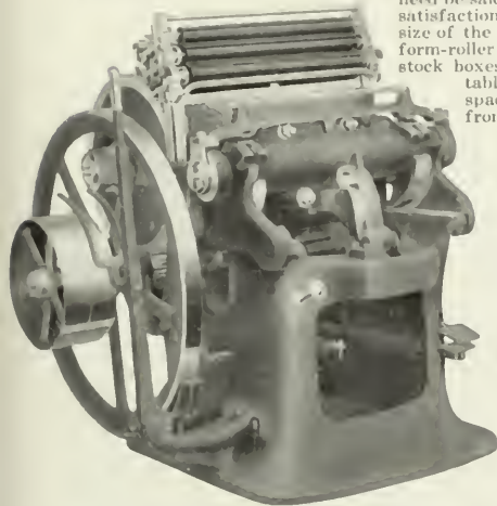
Colt's Armory, Style 2-A. Made in two sizes: Half Medium, 13x19 inches, and Half Super Royal, 14x22 inches (inside chase measurements).
