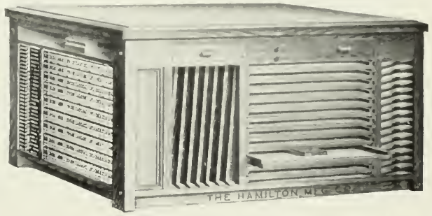
The Metropolitan Imposing Stone Frame. Showing one side and one end with open planner shelf and reglet and furniture racks. Recessed dustless base
