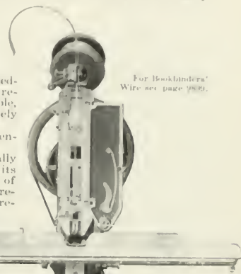
No. 7 Boston Wire Stitcher, showing door open. All working parts and wire always visible
