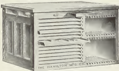
Ramaley Imposing Stone Frame. One view showing letter boards and chase racks
