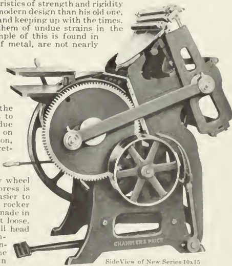
Side View of New Series 10x15 Chandler & Price Press
