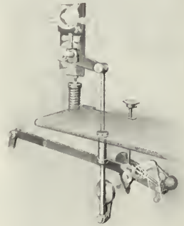
The Wonderful Eccentric Impression Mechanism—the span of a man's hand covers it.
