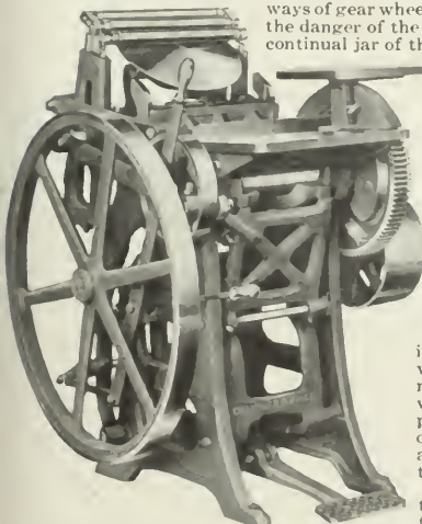
Three-Quarter View of an 8x12 New Series Chandler & Price Press
