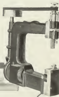
Miller Universal Saw-Trimmer with Router and Jig-saw Attachment
