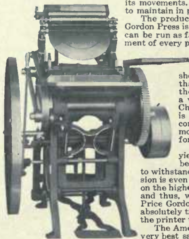
Chandler & Price Gordon Job Press Front View
