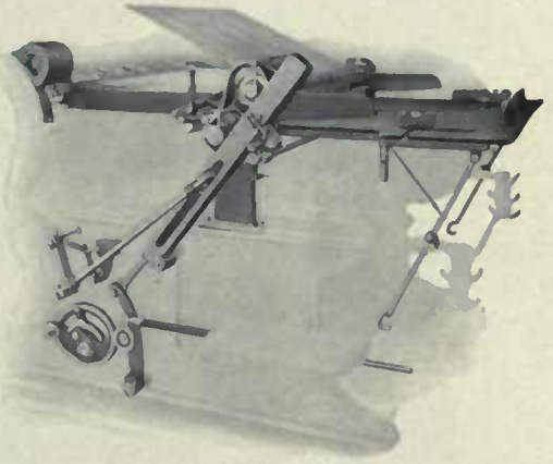
The Premier Fly Delivery
