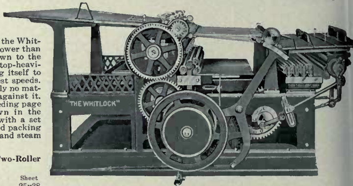
The Whitlock Pony, Front Fly Delivery
