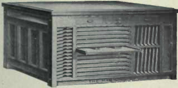
Metropolitan Imposing Stone Frame. Showing one side and one paneled end with planer shelf. Note the recessed base with rounded, dustless corners
