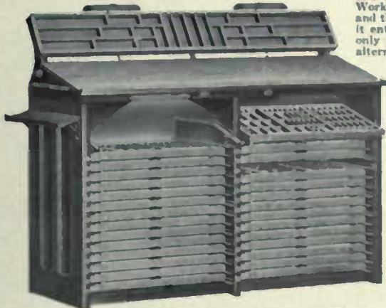
Mills Double Head Letter Cabinet, to hold 28 full size cases, and showing position of Linolite Lamps
