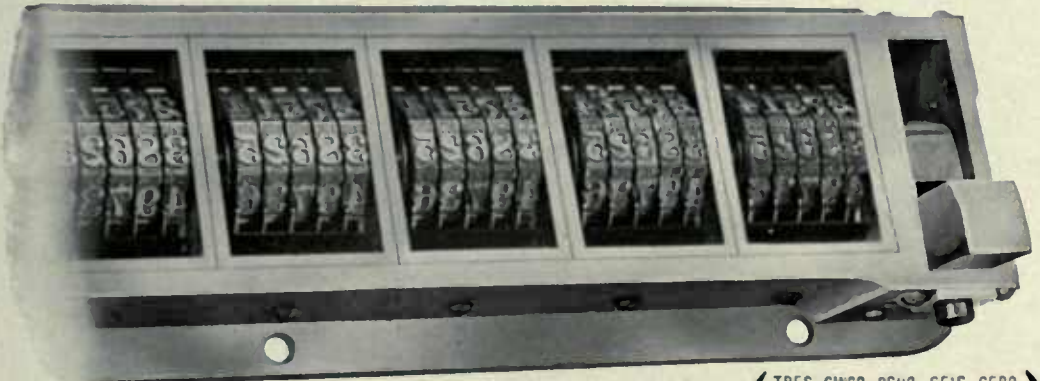
This illustration shows a section of a frame containing ten 5-wheel machines, which was designed to work on a 14x20 inch Gordon Press, and shows model 87 figures, with Spanish spelling above each figure.
