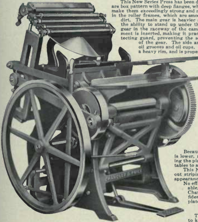
Three-Quarter View of 14½x22 New Series Chandler & Price Press
