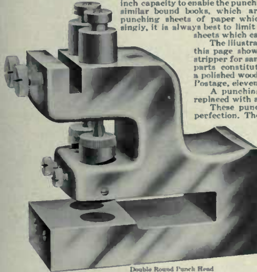
Double Round Punch Head
