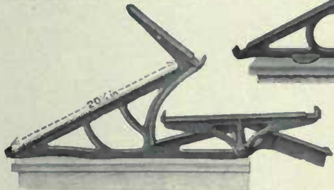
No. 3 Three-Case Tilting Bracket
