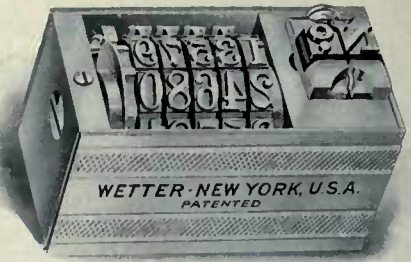
Wetter Model 125 Actual size 3/4x1 1/2 inches; consecutively numbers from 1 up to 99999. Prints figures like this impression
