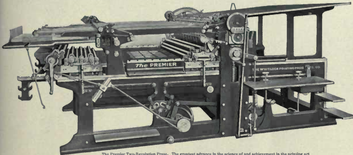
The Premier Two-Revolution Press. The greatest advance in the science of and achievement in the printing art
