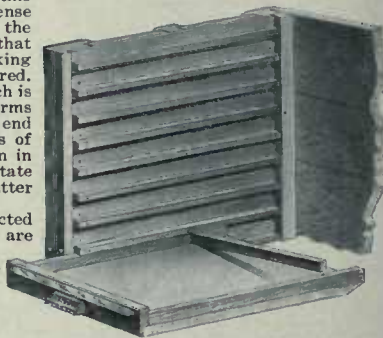
Detail showing construction of Page Form Storage Cabinet—Note Back Rail in Drawer
