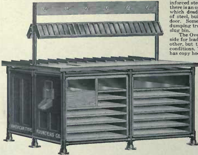
American Combination Dumping and Correcting Table No. 450
