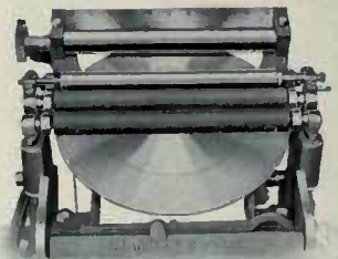
C. & P. Long Fountain with vibrating roller
