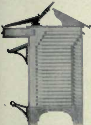
Sectional view of Masterman Composing Room Cabinet showing position of job cases, foot rail, supplementary galley bank, copy-drawer box and the brackets and 16x72 inch bank on top
