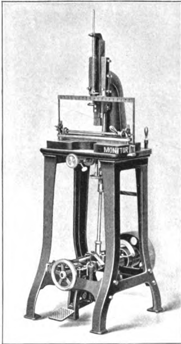
Complete, for Power, $180.00.
