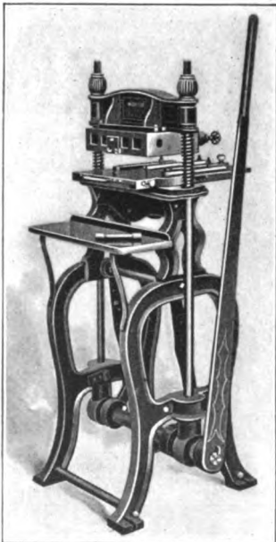
Monitor Lever Embosser No. 2.
