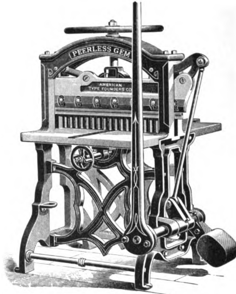
This illustrates the 30- and 32-inch Peerless Gem Paper Cutter, except that the balance weight is now hung inside the frame as shown in cuts of 23-inch size on next page.
