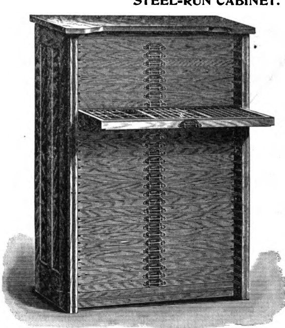
Shows construction of runs in Porter Cabinets. The steel runs are secured between wood, the wood screwed to sides, and two iron rods are passed through as extra strengtheners.
