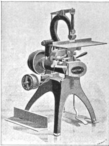
Power or Treadle.
