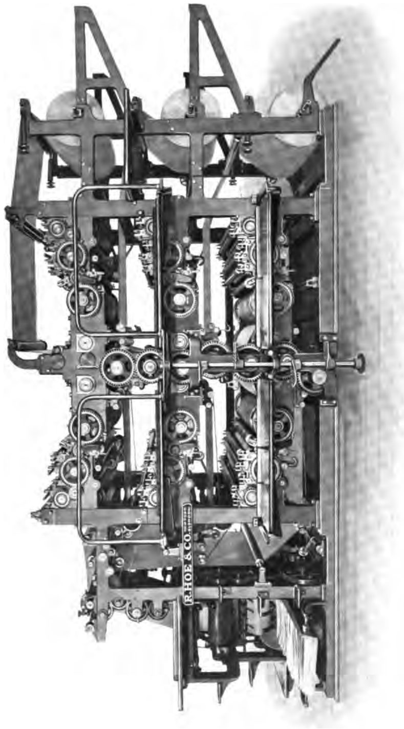
STRAIGHT-LINE PRESS
