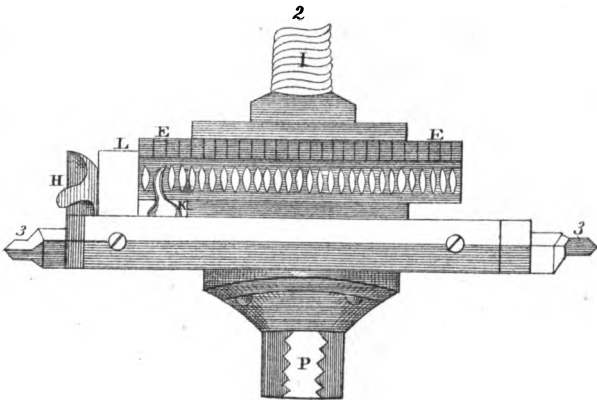
Eccentric Chuck
